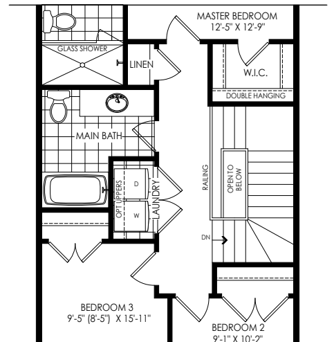
PARTIAL OPT. SECOND FLOOR PLAN W/ LAUNDRY ELEV 'WC2'
