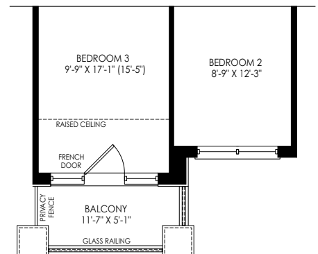
PARTIAL SECOND FLOOR PLAN ELEV 'WC1'
