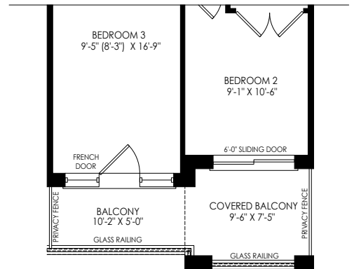
PARTIAL SECOND FLOOR PLAN ELEV 'M1'
