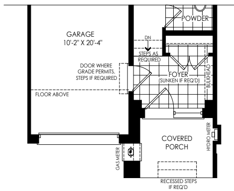
PARTIAL GROUND FLOOR PLAN ELEV 'WC3'
