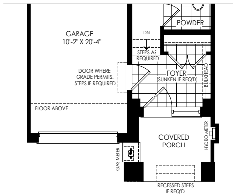
PARTIAL GROUND FLOOR PLAN ELEV 'M3'
