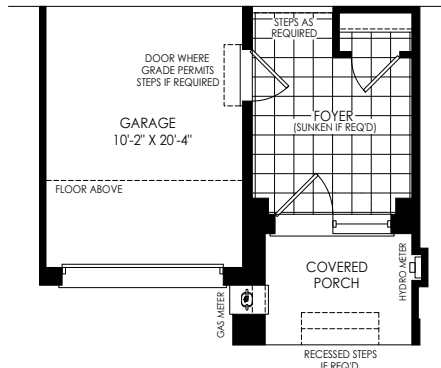
PARTIAL GROUND FLOOR PLAN ELEV 'WC3'
