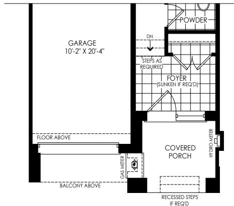
PARTIAL GROUND FLOOR PLAN ELEV 'M1'
