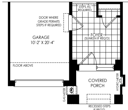
PARTIAL GROUND FLOOR PLAN ELEV 'M2'
