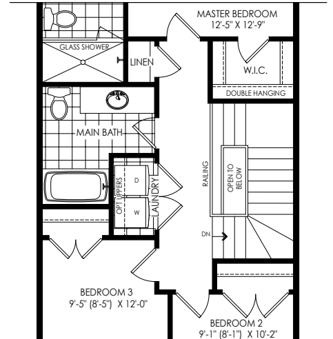
PARTIAL OPT. SECOND FLOOR PLAN W/ LAUNDRY ELEV 'T2', 'T4'
