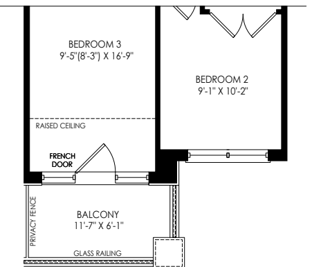
PARTIAL SECOND FLOOR PLAN ELEV 'WC2'
