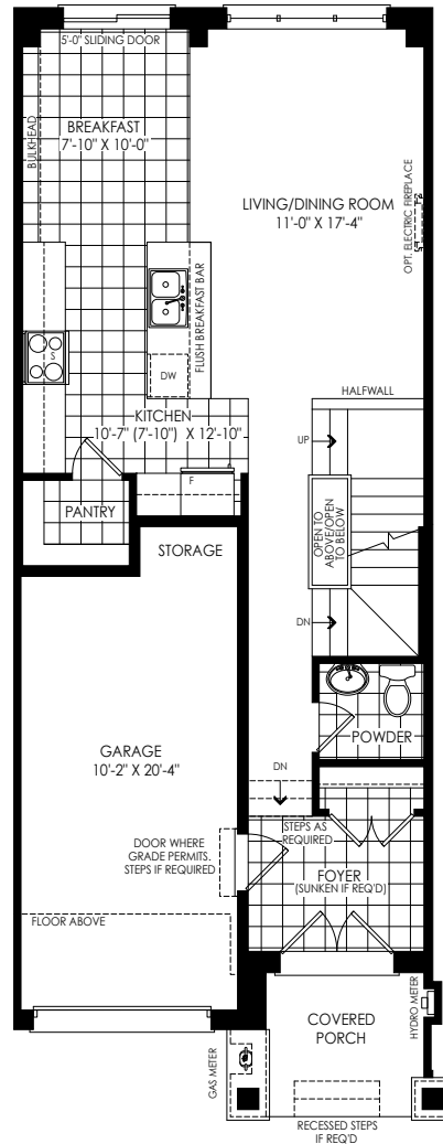
GROUND FLOOR PLAN ELEV 'T1'
