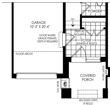
PARTIAL GROUND FLOOR PLAN ELEV 'WC4'
