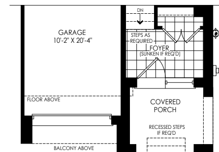
PARTIAL GROUND FLOOR PLAN ELEV 'M4'
