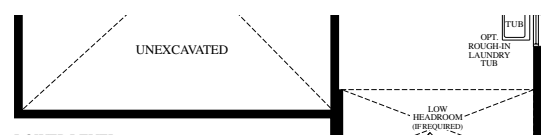
LOWER LEVEL ELEV. B
