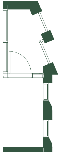
BALCONY ALTERNATIVE 603.605.621 EXTERIOR SIZE 42 ft 2
